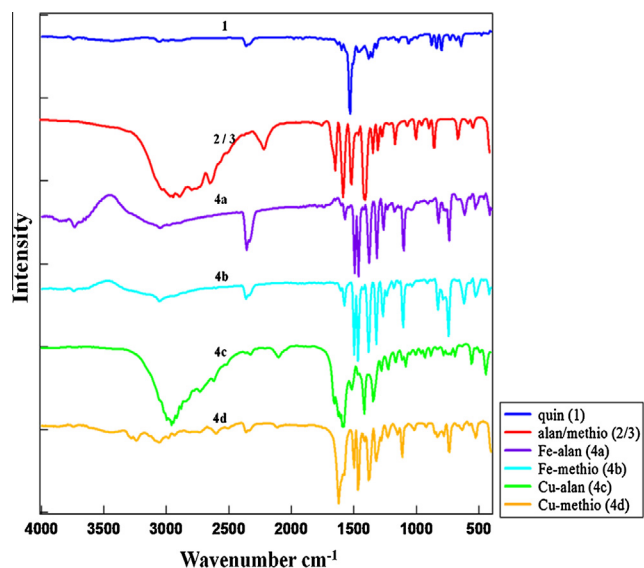
Figure 1 IR spectra of the ligands and complexes (4a–d).
