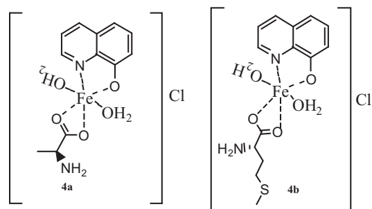
Figure 3a Iron octahedral geometry complexes.
