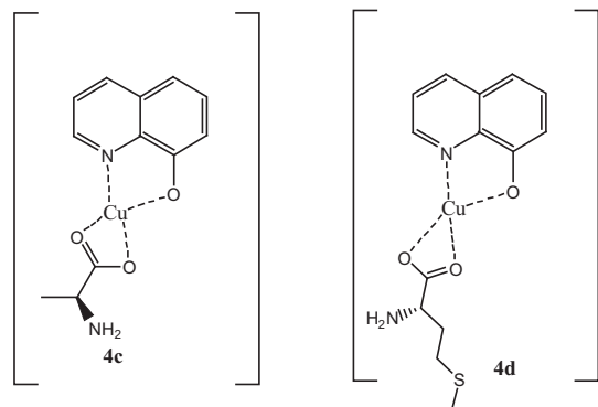
Figure 3b Copper tetrahedral geometry complexes.
