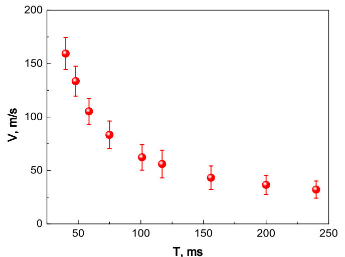
Fig. 2. The neutron velocity at the velocity selector exit is shown as a function of its rotation period. Error bars indicate the half width of velocity distribution in the beam after selector (these distributions are not Gaussians).
