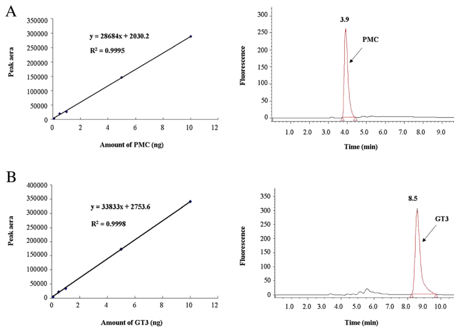
Figure 1 Calibration curves and chromatograms. HPLC calibration curves and chromatograms of PMC (A) and GT3 standard sample (B).
