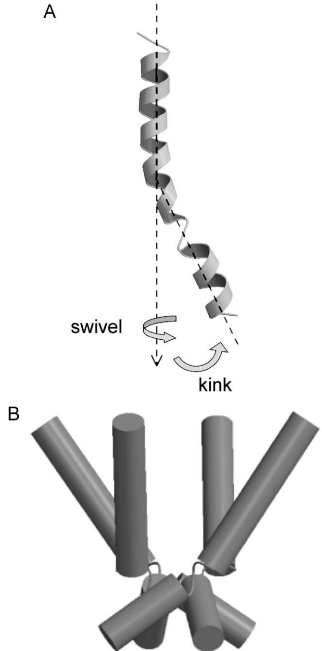
Fig. 12. (A) S6 helix structure taken from a simulation of the isolated helix in a membrane mimetic octane slab [110]. The N-terminus of the helix is at the top of the diagram. The definitions of helix kink and swivel angles are indicated. (B) Schematic model of the inner helix bundle of Kv channel pore as formed by four kinked S6 helices.
