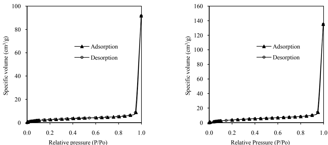
Fig. 3. Sorption isotherm of char obtained from fast pyrolysis of plastic wastes (a) without activation; (b) with activation under air atmosphere at 900°C for 3 hours.
