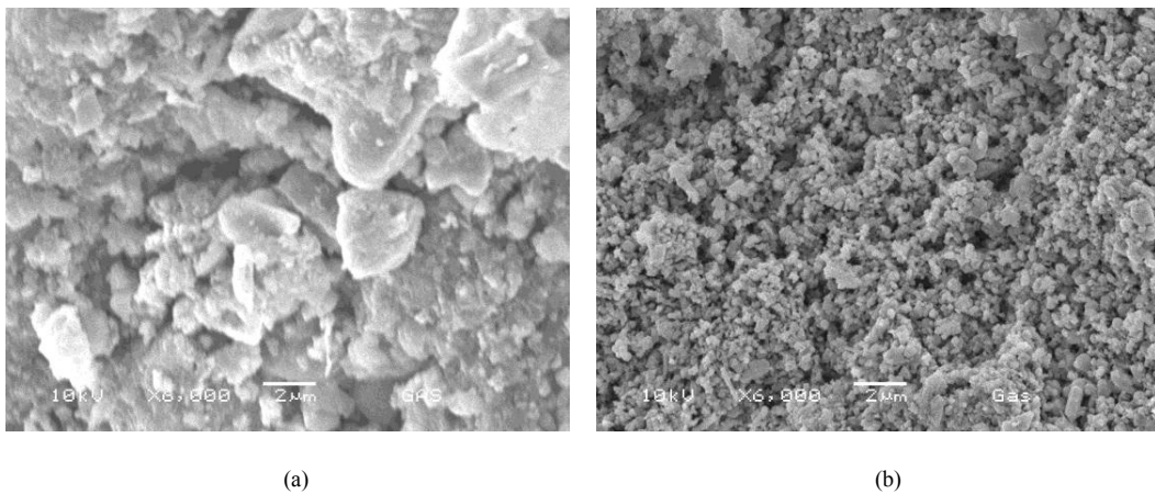
Fig. 2. Micrograph of chars derived from gasification of plastic wastes (a) without activation; (b) with activation under air atmosphere at 900°C for 3 hours.
