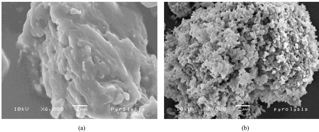
Fig. 1. Micrograph of chars derived from fast pyrolysis of plastic wastes (a) without activation; (b) with activation under air atmosphere at 900°C for 3 hours.
