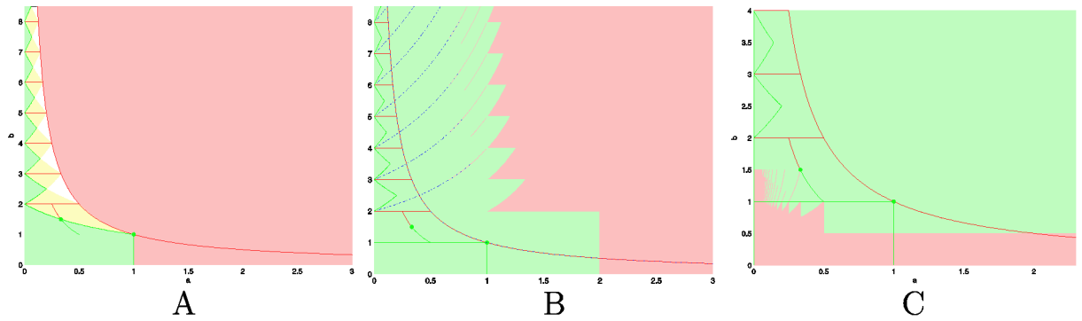
Fig. 2. (A) Janssen tie, i.e., set containing pairs (a, b) , a, b > 0 , such that (\mathbf{1}_{[0,1]}, a, b) is not a frame (dark), set containing pairs (a, b) , a, b > 0 , such that (\mathbf{1}_{[0,1]}, a, b) is a frame (white). In the light area, it is known that (\mathbf{1}_{[0,1]}, a, b) is a frame if ab is irrational. (B) Superposition of Janssen tie and Fig. 1.B. (C) Superposition of Janssen tie and Fig. 1.C.
