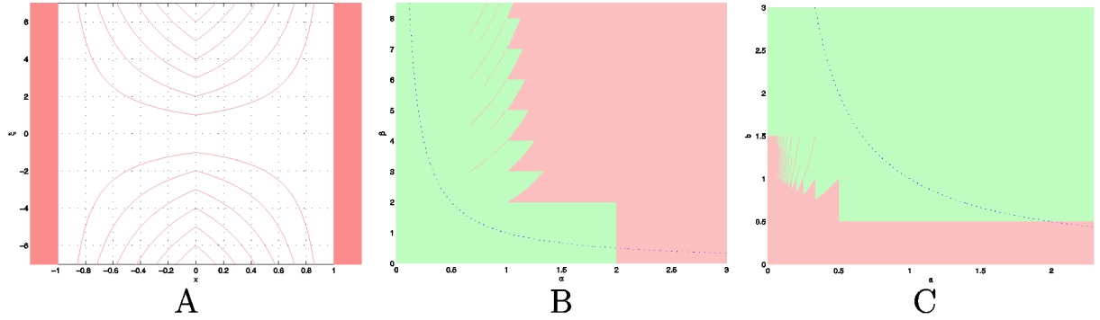
Fig. 1. (A) Zero set of V_{\mathbf{1}_{[0,1]}} \mathbf{1}_{[0,1]} (dark). (B) Set containing all pairs (\alpha, \beta) , \alpha, \beta > 0 such that P_{\alpha\mathbb{Z} \times \beta\mathbb{Z}} |V_g g|^2 has a root (dark). We include as reference the curve \alpha\beta = 1 (dashed). (C) Set containing all pairs (a, b) , a, b > 0 such that \{\rho(an, bm) P_g\}_{n,m \in \mathbb{Z}} is not a Riesz basis in HS(\mathbb{R}) (dark). The curve ab = 1 is included (dashed).
