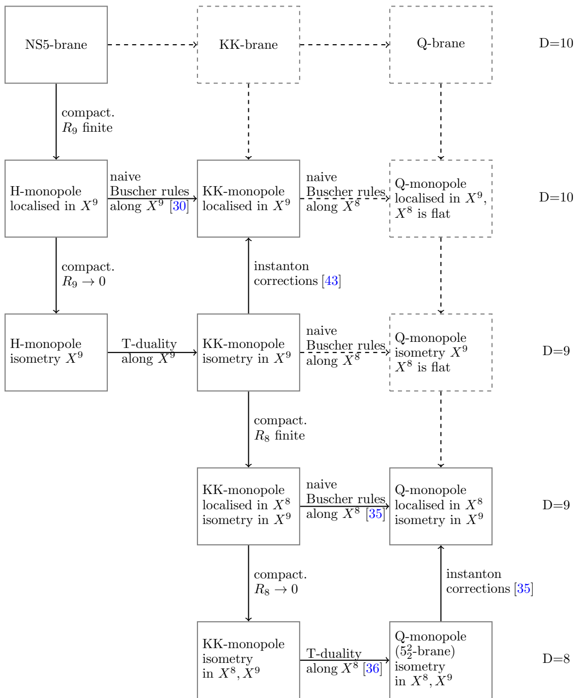
Figure 1. Systematics of backgrounds with H, geometric \tau and Q fluxes and their relations. Note that in [35] Q-monopole localised in both X^8 and X^9 has been constructed with both these directions being compact.
