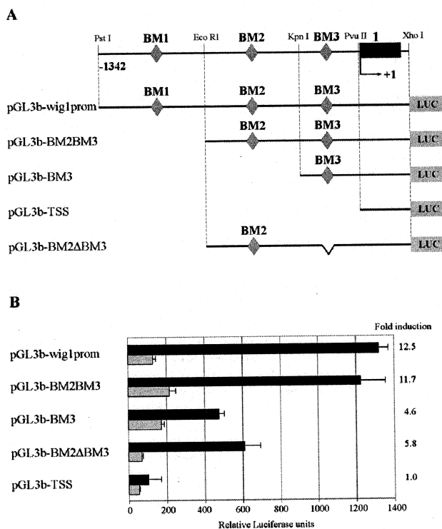
Fig. 3. A: A schematic representation of the luciferase reporter constructs used. Restriction sites used for cloning are indicated. B: p53 -/- MEFs were cotransfected with 1 μg of indicated luciferase reporter and 0.5 μg wtp53 (black) or mt p53(175) (gray) plasmid. The data are representative of three independent experiments, each performed in triplicates after normalization with β-galactosidase activity and protein concentrations.
