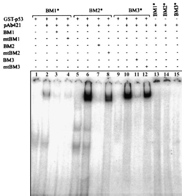
Fig. 2. EMSA showing binding of p53 to the p53-binding motifs in the wig-1 promoter in vitro. Recombinant p53 protein (50 ng) incubated with [ \alpha - 32 P]ATP-labeled oligonucleotides corresponding to the three p53-binding sites. The p53–DNA complexes were resolved on a 4% native polyacrylamide gel. For competition, 10-fold excess of unlabeled oligonucleotides was added to the reactions. The p53 antibody PAb421 was added to activate recombinant p53.
