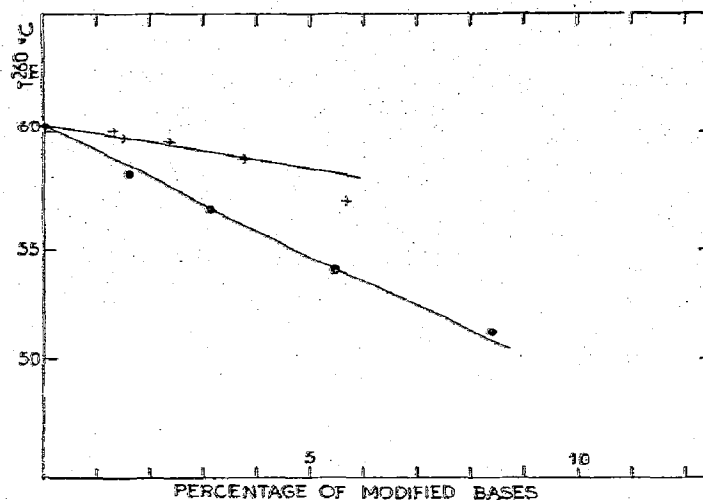
Fig. 2. Melting temperature at 260 nm vs. percentage of modified bases in 2 \times 10^{-3} M/l sodium citrate buffer (pH 7). +: DNA-AAIF. •: DNA-AAF. The decrease of T_m^{260} with AAFF modified DNA is similar to that observed with DNA-AAF.
