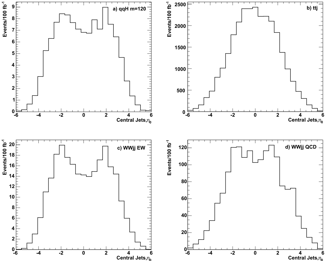
Fig. 3. \eta_0 = \eta_3 - (\eta_1 + \eta_2)/2 for the third jet. \eta of the third jet with respect to the average of the two forward jets. For signal (a) qqH , m_H = 120 GeV and backgrounds (b) t\bar{t}j , (c) EW WWjj and (d) QCD WWjj
