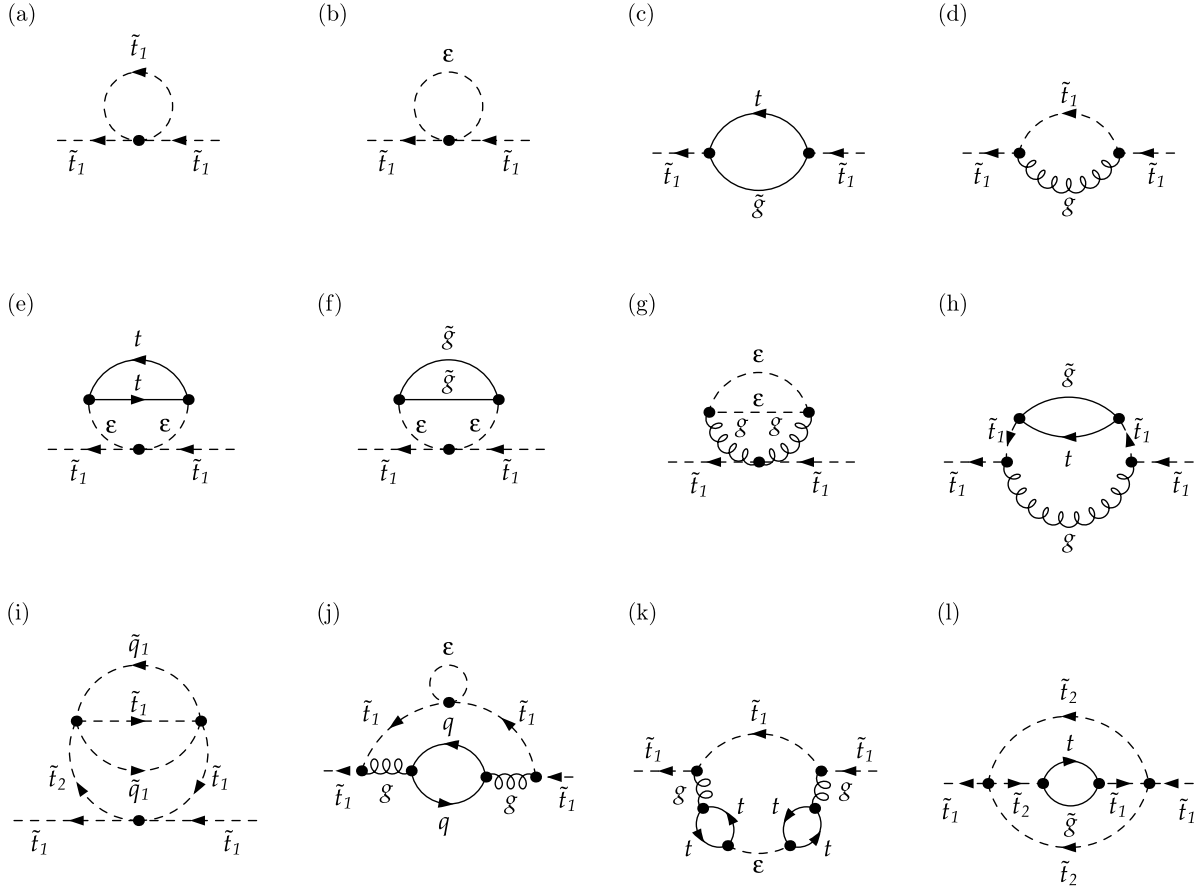
Fig. 1. Sample diagrams contributing to \Sigma_{11} at one, two and three loops. The symbols t , \tilde{t}_i , g , \tilde{g} and \epsilon denote top quarks, top squarks, gluons, gluinos, and \epsilon scalars, respectively.
