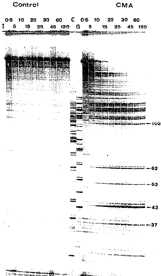
Fig. 1. Transcriptional blockages induced by CMA. The drug (1 μM) was reacted with initiated transcription complexes in transcription buffer (pH 8.0) at 37°C for times ranging from 0.5 to 120 min. The initiated complex is shown in lane I, while C and G denote sequencing lanes where transcription was terminated by methoxy-CTP and methoxy-GTP, respectively [16-18]. The control lanes represent elongation of the initiated complex in the absence of added drug.
