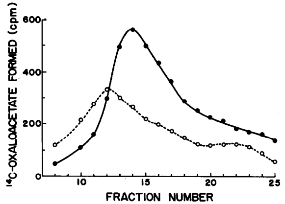
Fig. 2. DEAE-Sephadex column chromatography of PEP carboxykinases from control adult chicken. Protein amounts applied, the assay conditions, and the signs were the same as for expt. 1 in fig. 1.
