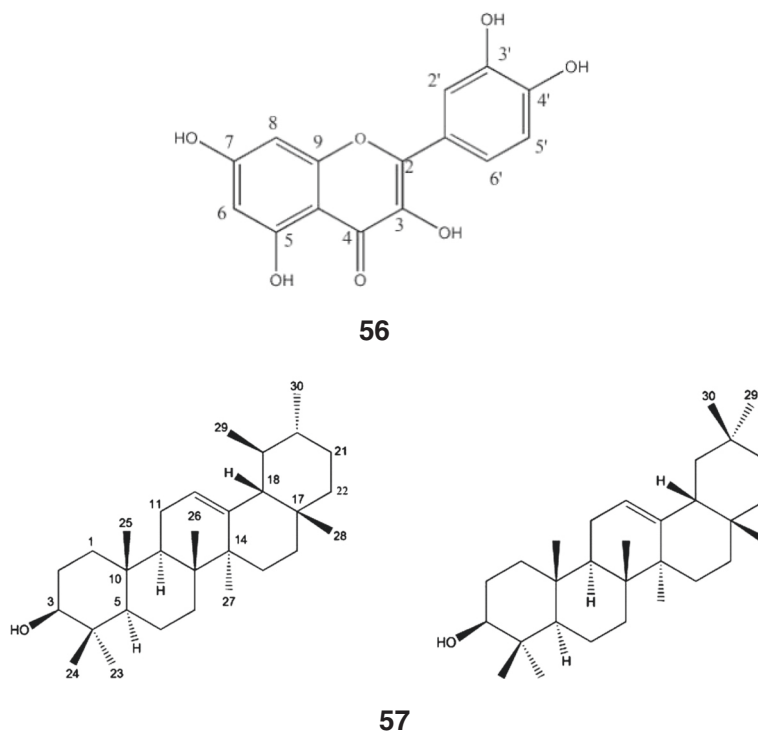
Fig 1 The chemical structures of quercetin ( 56 ) isolated from the chloroform soluble fractions of Duranta repens flowers and \alpha - and \beta -amyrin ( 57 ) isolated from the hexane extract of Ixora coccinea flowers
