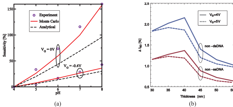
Fig. 4. (a) Comparison between experimental and simulated data. The sensitivity as a function of pH value of the electrolyte is calculated for gate voltages of 0V and -0.4V. The Monte-Carlo method outperforms the analytical model. (b) Current change, when molecules are detected, as a function of the nanowire thickness when ssDNA or dsDNA are present at the surface.
