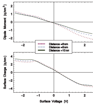
Fig. 3. Dipole-moment density and surface-charge density for different distances between dsDNA strands as a function of the surface voltage.
