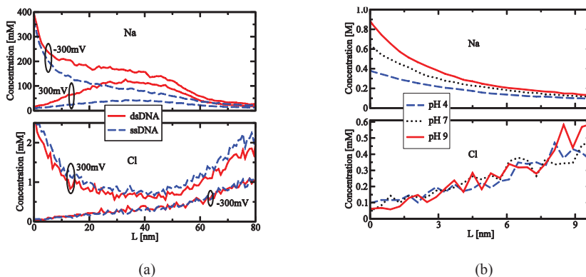
Fig. 2. (a) Na + and Cl - concentration profiles with ssDNA and dsDNA immobilized on the surface at electrolyte voltages of -300mV and +300mV. (b) Ion concentration profile as functions of the distance from the surface at a surface voltage of -0.4V for different pH values.
