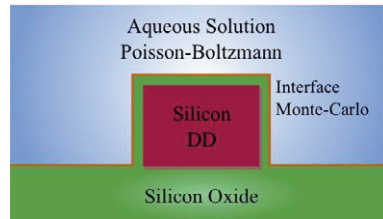
Fig. 1. Schematic cross section of the nanowire biosensor. The silicon nanowire is described by the drift-diffusion model, while the interface and the surface layer in the electrolyte are modeled by a Monte-Carlo approach.
