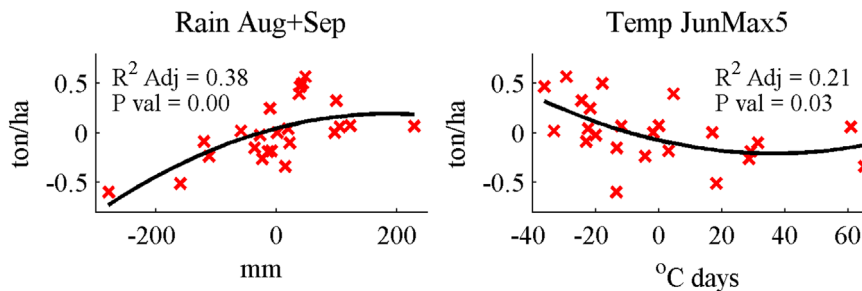
Fig. 9. Bol millet yield bivariate correlations (1st-order difference).
