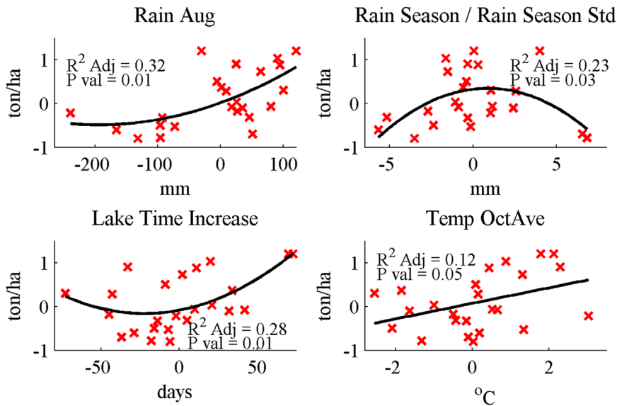
Fig. 10. Doum-Doum maize yield bivariate correlations (1st difference).
