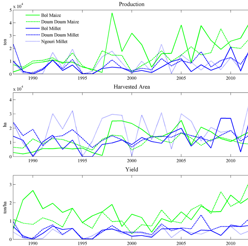
Fig. 5. Production, harvested area and yield for maize & millet per rainy season and sub-region.
