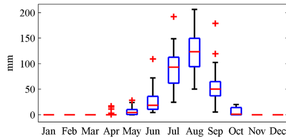
Fig. 2. Monthly rain boxplot (region average).
