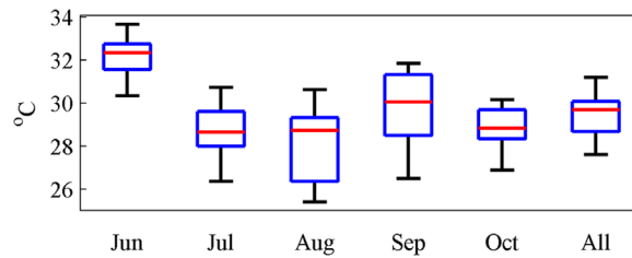
Fig. 4. Distribution of monthly average temperatures in Bol.
