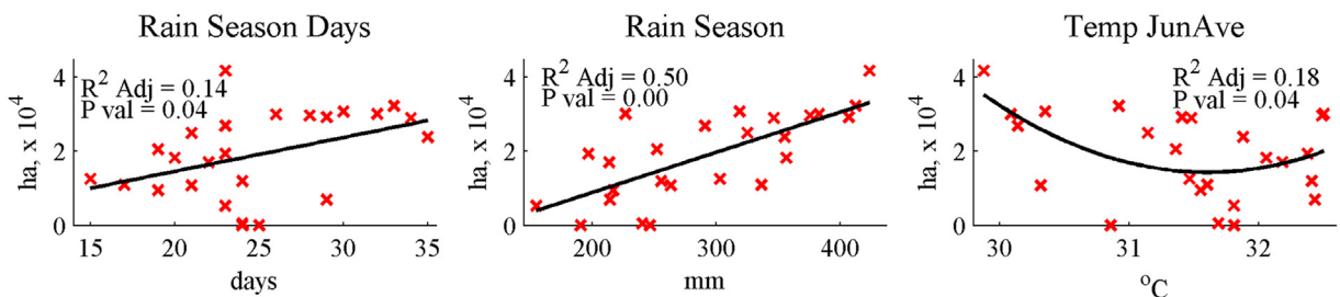
Fig. 13. Ngouri millet harvested area bivariate correlations.
