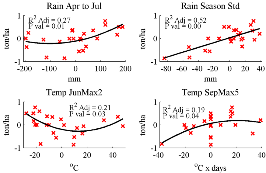
Fig. 12. Doum-Doum millet yield bivariate correlations (1st-order difference).
