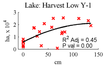
Fig. 6. Bol maize harvested area bivariate correlation.
