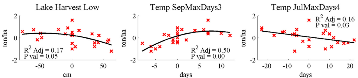
Fig. 7. Bol maize yield bivariate correlations (1st-order difference).
