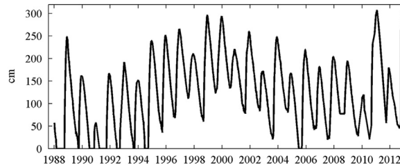
Fig. 3. Lake Chad water depth measured at Bol 1988–2012 (daily).
