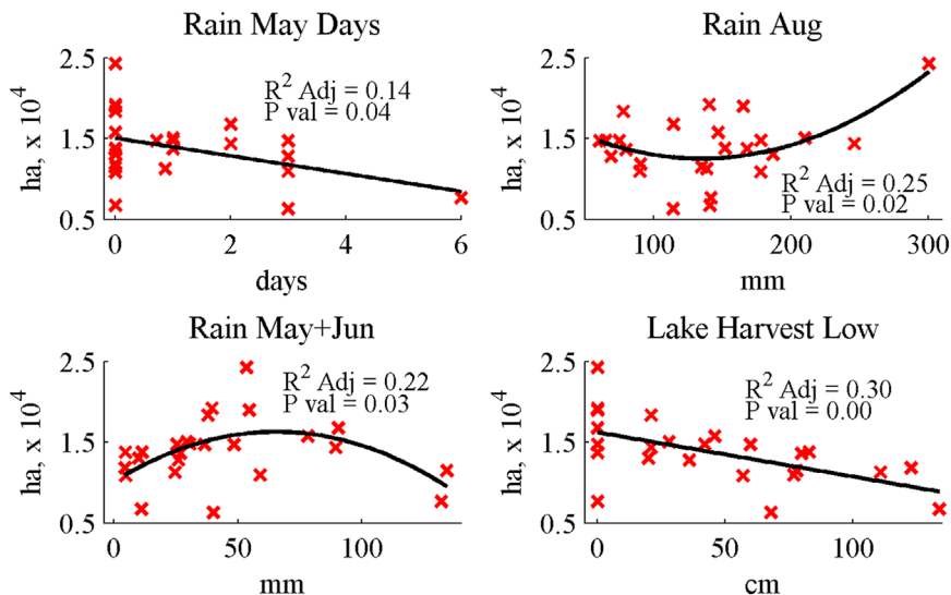
Fig. 11. Doum-Doum millet harvested area bivariate correlations.
