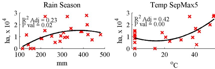
Fig. 8. Bol millet harvested area bivariate correlations.
