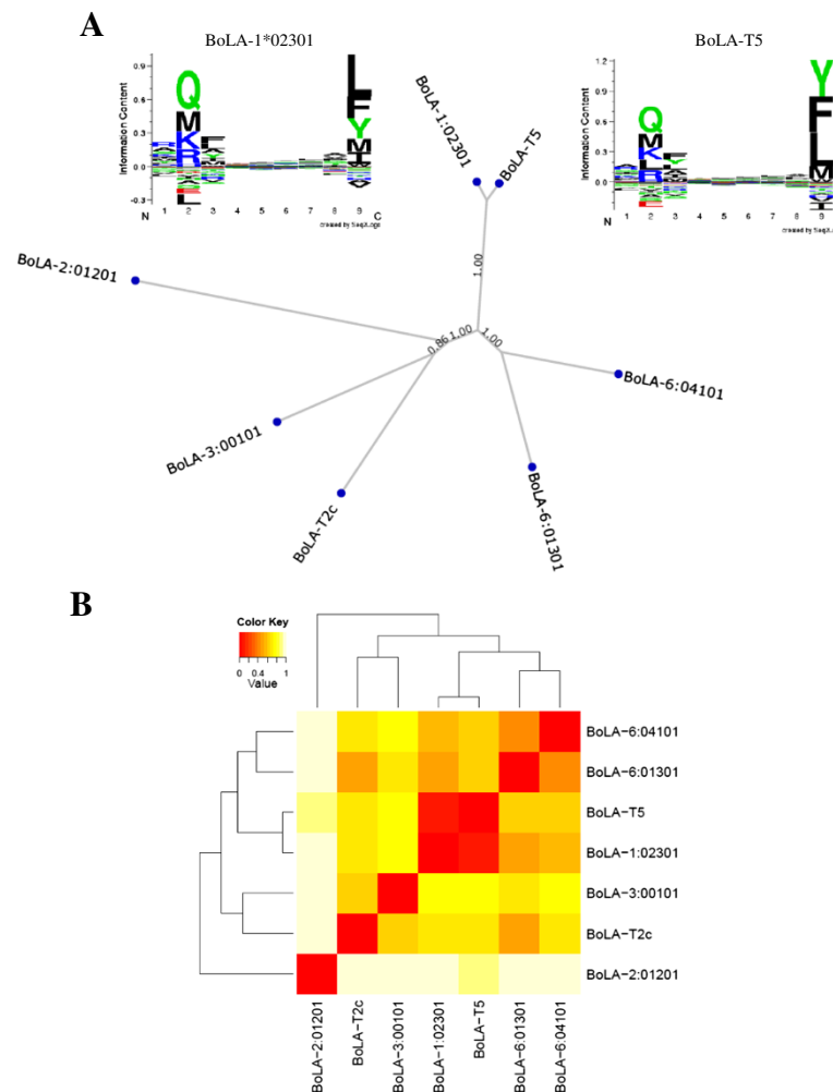
Figure 6 MHCcluster prediction of the functional similarity of BoLA-T5 and BoLA-1*02301. Panel A : UPGMA tree-based clustering of the relationship between the seven BoLA molecules (sequence logo representations of the predicted binding motifs of BoLA-T5 and BoLA-1*02301 were generated by MHCcluster using Seq2Logo [52]); Panel B : heat-map visualization of the degree of functional relationship between the seven BoLA molecules, red colour shows closer functional relationship.
