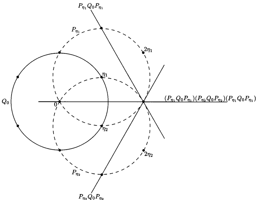
FIG. 5.1. A 2-dimensional section of \text{Im } \mathbb{O} (see the Proof of Theorem 5.3). Dots indicate elements of \text{Im } \mathcal{H} . The real reflection Q_0 acts by inversion in the solid circle. The lines are the mirrors of certain other real reflections, whose names are next to them. Each dashed circle is carried to itself by the octave reflection whose name is next to it; this reflection carries each point on the dashed circle to its antipode on the same dashed circle. The octave reflection also exchanges the center of the dashed circle with \infty .
