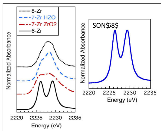
Fig. 1. Left. Zr-L 2,3 XANES spectra of crystalline references, lemoynite ((Na,K) 2 CaZr 2 Si 10 O 26 · 5–6H 2 O) ( 16 Zr), baddeleyite (m-ZrO 2 ) and hydrous zirconia (HZO) (both with 171 Zr) and ZrSiO 4 ( 181 Zr). Right. Zr-L 2,3 XANES spectrum in SON68 glass.
