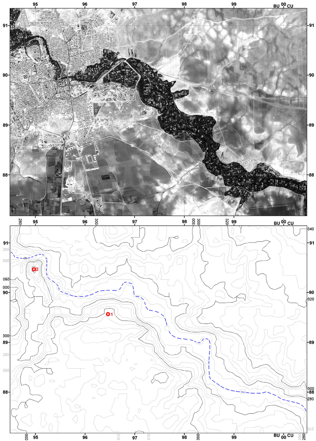
Fig. 9. Paired images showing the M. meridionalis locality at Sharia, Hama: upper – GAMBIT image, taken in 1967; lower SRTM-derived contour image, with selected 5 m interval contours labelled and the Sharia locality indicated, centre left (as Point 1) in what was in 1967 the south-eastern edge of the Hama conurbation (UTM coordinates: BU 965 896). Point 2 is the ancient citadel in the centre of Hama. Coordinates are marked for 1 km grid squares.
