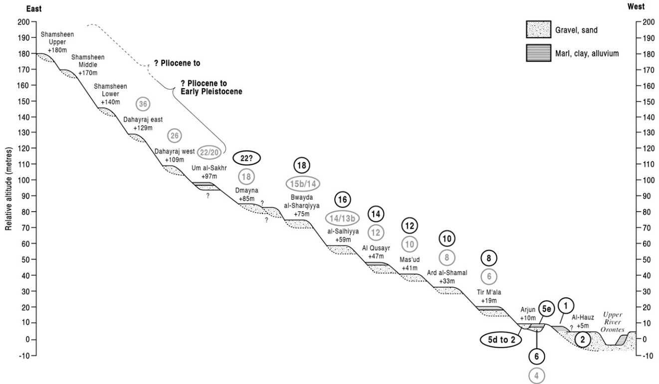
Fig. 4. Idealized transverse section through the terrace sequence upstream from Homs (after Bridgland et al., 2003, with modifications). MIS attributions suggested by Bridgland et al. (2003) are shown, together with correlations of the older terraces now suggested (see text).
