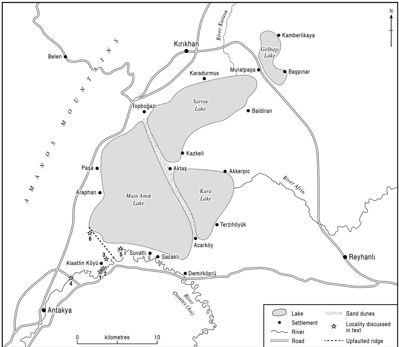
Fig. 13. The Amik basin showing the extent of the former Lake Amik (modified from Çalıışkan, 2008). For location, see Fig. 1. Field localities are numbered as follows (see text): 1, the Alaattin Köyü clast analysis locality (see Table 1); 2, river-bank Section 1 km south of Alaattin Köyü (BA 52477 15506); 3, quarry section in upfaulted basin sediments at Alaattin Köyü (BA 52626 16772); 4 and 5, downstream and upstream limits of measurement fluvial entrenchment beneath the Amik Plain (at BA 48448 15139 and BA 54539 18533, respectively); 6, spot-height in the upfaulted sediment observed at 3, at 159 m a.s.l. (~BA 508 200).
