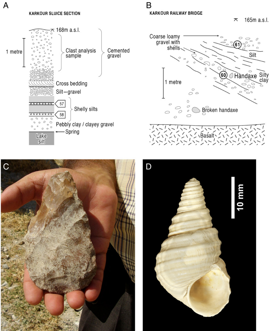
Fig. 11. Karkour, northern Ghab Basin: A – Section log from the Karkour sluice locality; B – Section log from the Karkour railway bridge locality; C – hand axe from the Karkour railway bridge section; D – Apameus apameae from the Karkour railway bridge section. This species is named after Apamea, a Roman site in the Ghab.
