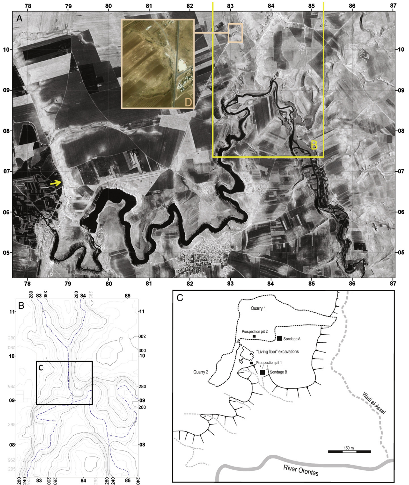
Fig. 8. The important archaeological and fossiliferous locality at Latamneh: A – CORONA image from the 1960s of the area between Latamneh and the Sheizar fault scarp, the latter being indicated with an arrow (top left); the southern part of Latamneh village is at the northern edge of this image, within the area of B. B – Contour map (5 m interval) derived from Shuttle Radar Topographic Mission (SRTM). C – Location of the earlier palaeontological and archaeological localities at Latamneh (from Shaw, in press ). D – Inset showing a modern Google Earth view of the extant quarry at Latamneh, to the north of the earlier localities depicted in C.
