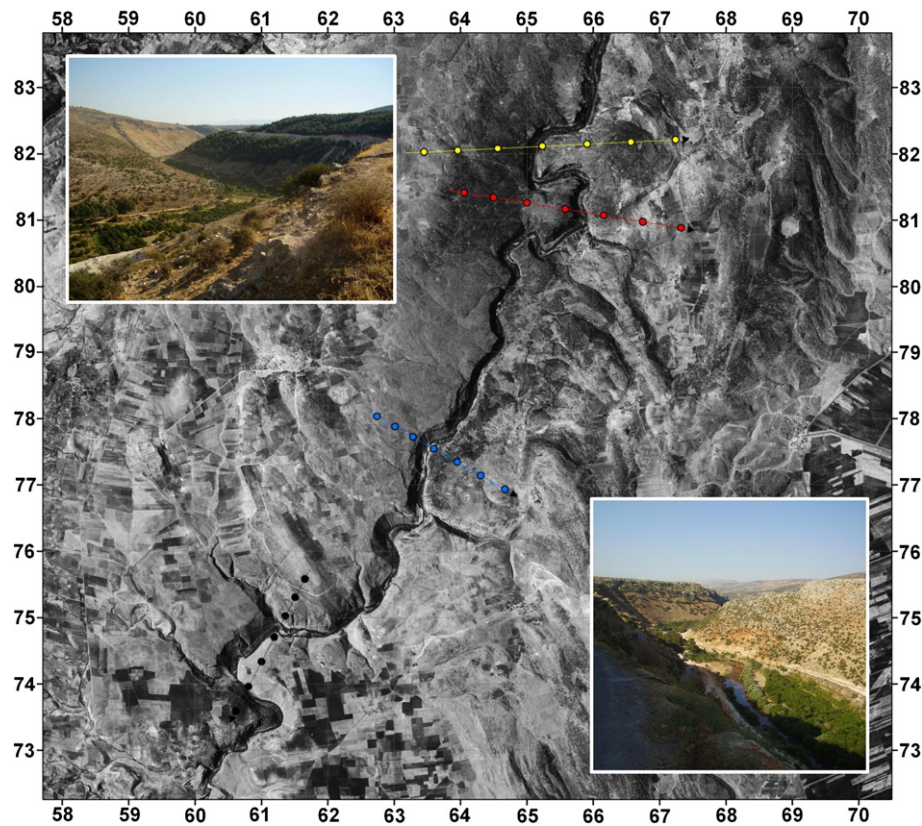
Fig. 12. The gorge between Jisir ash-Shugour and Darkush: 1960s CORONA image of the gorge (for location, see Fig. 1); dotted lines show locations of derived cross sections (see online supplement, Fig. A.1.9). Coordinates are marked for 1 km grid squares. Insets show photographic images of the gorge: A – looking SSW (upstream) from BV 63205 76708, about 5 km east of Qanaya. The mountains visible in the far distance are part of the Jebel Nusayriyah range along the western side of the Ghab Basin.; B – Looking northwards, downstream along the valley, from BV 63234 76771. The gravel sample locality at Hammam ash Shaykh Isa is ~400 m to the north of the viewpoint, accessed from the nearer part of the valley-floor platform in the middle distance. Both photographs show features that might represent early river levels, although other explanations would be possible and ground-truthing has not been practicable.
