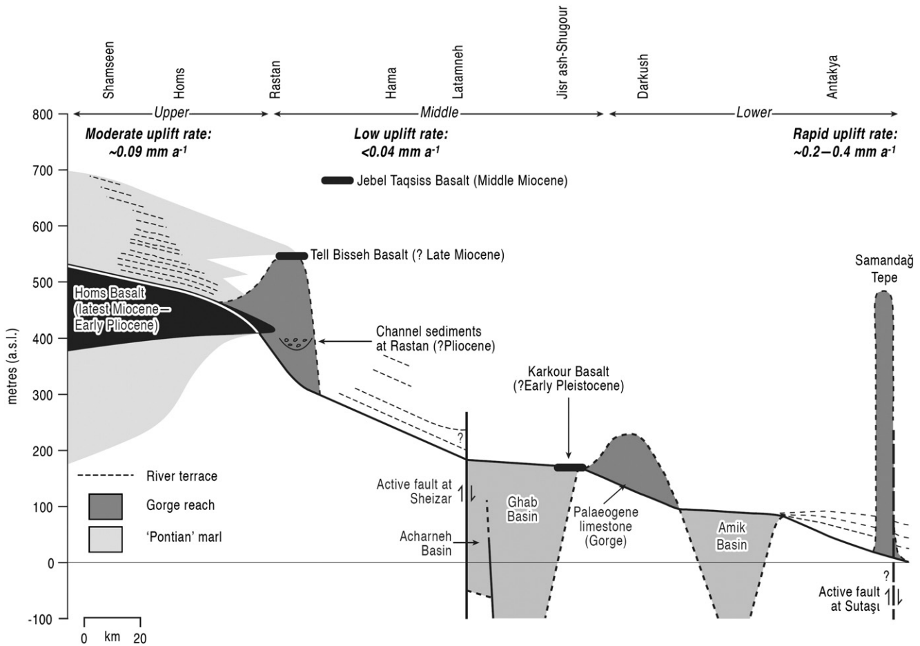
Fig. 3. Schematic long profile of the Orontes valley floor and its terraces in relation to gorge reaches, subsiding fluvio-lacustrine basins and basalt flows. Summaries of post-Early Pleistocene histories of the terraced reaches are also shown (for explanation, see text).
