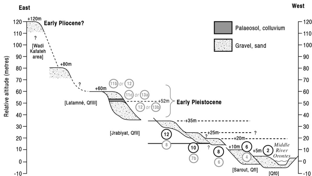
Fig. 7. Idealized transverse section through the terrace sequence of the Hama-Latamneh area, showing the MIS correlation suggested by Bridgland et al. (2003), now thought to be underestimated, and the greater ages suggested in this paper (see text). Uses data from Besançon and Sanlaville (1993a) and Dodonov et al. (1993); artwork modified from Bridgland et al. (2003).
