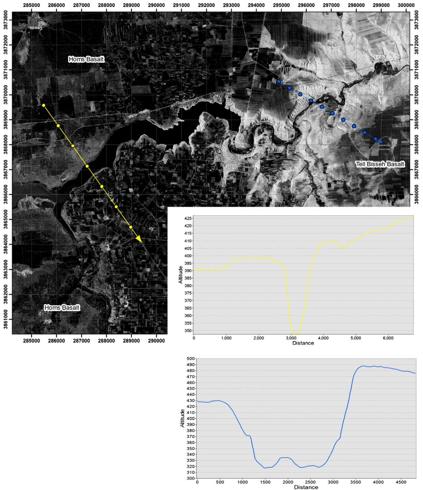
Fig. 5. The Rastan Gorge. This is a CORONA image from the 1960s, with derived transverse profiles (colour coded). Positions of the two basalts, of different age, are indicated (see text). The westernmost (upper) cross section is located on the Homs Basalt on both sides of the river, whereas the easternmost (lower) cross section shows the higher Tell Bisseh Plateau on the right bank of the river.
