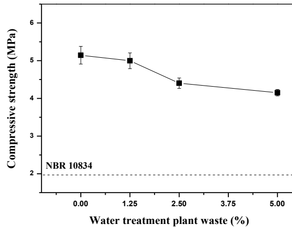
Fig. 2. Compressive strength of the soil-cement.
