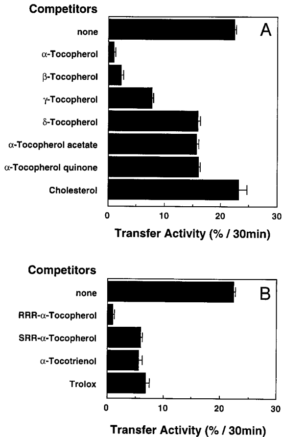
Fig. 3. Effect of the incorporation of unlabeled tocopherol analogs into liposomes on the transfer of \alpha - ^3\text{H} tocopherol. Liposomes composed of egg yolk phosphatidylcholine, bis(hexadecanyl)-phosphate and chromanol (A) or side chain (B) analogs of \alpha -tocopherol (molar ratio 10:1:0.16, 0.07 \mu\text{mol} phospholipid/tube) with traces of radioactive \alpha -tocopherol ( 5.7 \times 10^4 dpm) were incubated with membranes at 37^\circ\text{C} for 30 min in the presence of 40 ng purified \alpha\text{TTP} . Each point denotes the means \pm SE of three experiments.
