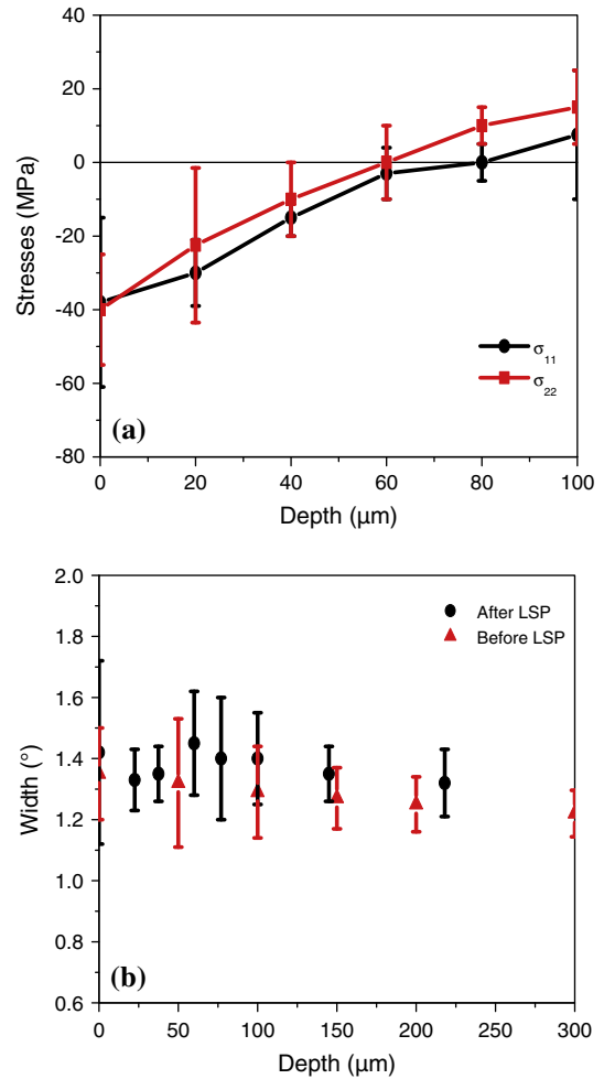
Fig. 6. (a) Initial residual stresses of AA2050-T8, \sigma_{11} (rolling direction) and \sigma_{22} (transverse direction), (b) influence of LSP on the integral widths of X-ray peaks (5 GW/cm 2 – 50% overlap).
