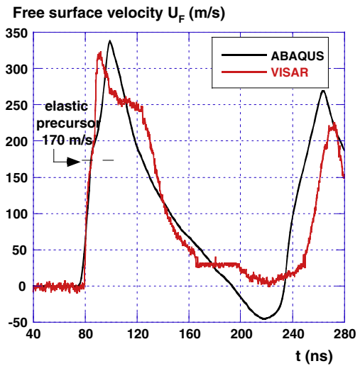
Fig. 5. Determination of the elastic precursor (inflexion at 170 m/s) and shock yield stress using back free velocity U_f measurements on a 430 μm-thick 2050-T8 foil ( I = 5.5 \text{ GW/cm}^2 , surface pressure = 3.8 GPa)–comparison with Abaqus simulation.
