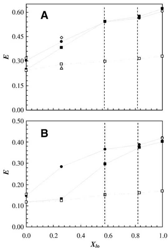
Fig. 5. Variation of FRET efficiency, E , for the D/A pairs (A) t -PnA/ N -NBD-16:0, 16:0 PE (D/A 2), and (B) t -PnA/ N -NBD-18:1, 18:1 PE (D/A 3) as a function of X_{lo} , in the l_o/l_d coexistence region along the tie line of the ternary phase diagram for the 16:0,18:1 PC/PSM/Chol mixture [75] containing 0 (circles) and 4 (squares) mol% PCer. Experimental data are represented by solid symbols, and open symbols are values from theoretical calculations. The open circles were obtained by calculation of the expected E for a random distribution of donors and acceptors. The open squares correspond to the expected E when donors located both in the gel and fluid phases are transferring energy to acceptors randomly distributed in the fluid phases. In these calculations a gel phase mole fraction X_G equal to 15% and R_e = 3.8 and 4.0 nm for N -NBD-16:0,16:0 PE and N -NBD-18:1, 18:1 PE, respectively, were assumed. The open triangle and the open diamond (A) correspond to the expected E for a situation where PCer/PSM gel domains are surrounded by only l_d or l_o phases, respectively. It was assumed that donors located in the gel phase were only able to transfer to one of the fluid phases, X_G = 15\% , R_e = 3.8 nm, and the amount of donor in the gel phase and the surface density of the acceptors in each fluid phase was taken into account. The dotted and dotted-dashed lines are only to guide the eye. The vertical dashed lines correspond to the mixtures containing 25% and 33% Chol. Time-resolved FRET measurements are extremely reproducible, and variations in the values of E are within < 1.5% for completely independent samples. Adapted from [88].
