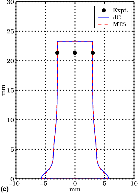
Fig. 18. Comparison of MTS and JC predictions of final Taylor specimen profiles with experimental results. (a) Case 1, (b) case 2, (c) case 3 and (d) case 4.
