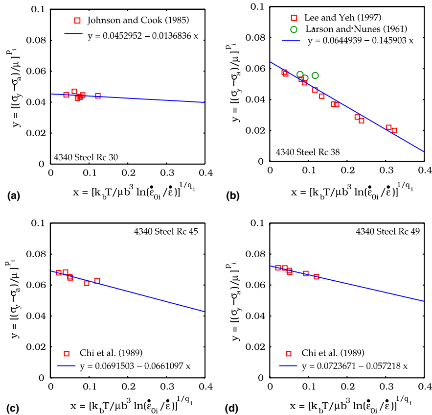
Fig. 1. Fisher plots for the intrinsic component of the MTS model for various tempers of 4340 steel. Experimental data are from Larson and Nunes (1961), Johnson and Cook (1985), Chi et al. (1989), and Lee and Yeh (1997). \sigma_a = 50 MPa, p_i = 2/3 , q_i = 1 , \dot{\epsilon}_{0i} = 10^3 s ^{-1} , k_b = 1.3806503e-23 J/K, b = 2.48e-10 m. (a) R_c = 30 , (b) R_c = 38 , (c) R_c = 45 and (d) R_c = 49 .
