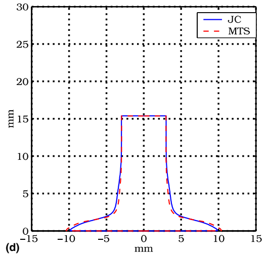
Fig. 18. Comparison of MTS and JC predictions of final Taylor specimen profiles with experimental results. (a) Case 1, (b) case 2, (c) case 3 and (d) case 4.
