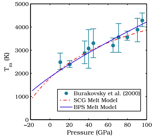
Fig. A.2. Comparison of experimental data and model predictions of the melting temperature of iron as a function of pressure. The experimental data are from Burakovskiy et al. (2000a).
