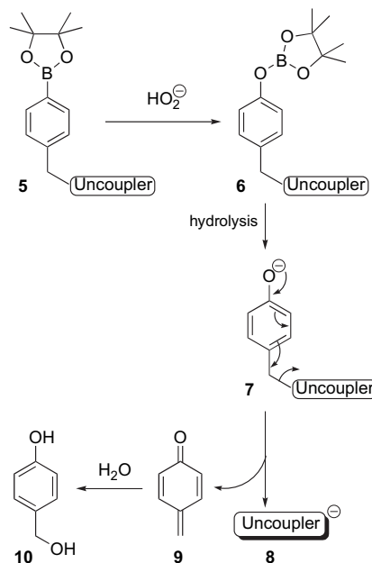
Scheme 2. Reaction between caged uncouplers and hydrogen peroxide.
