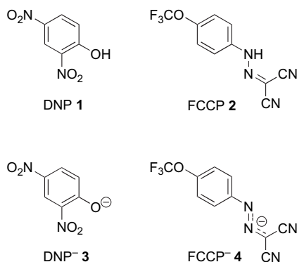
Figure 1. Uncouplers in their protonated and unprotonated forms.
