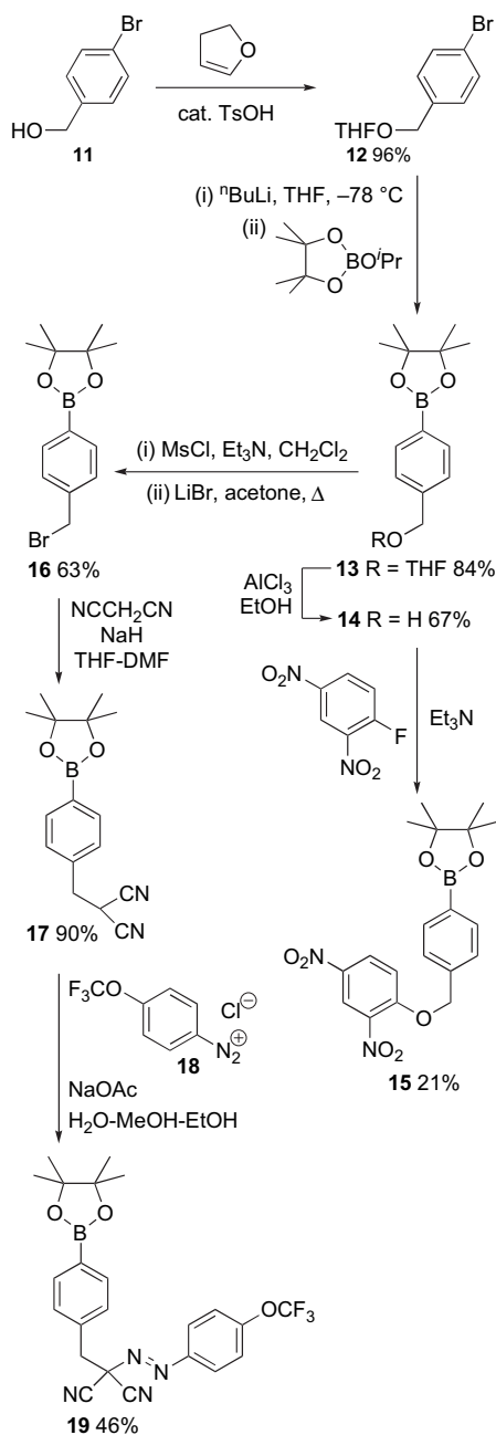
Scheme 3. Synthesis of caged uncouplers 15 and 19 .
