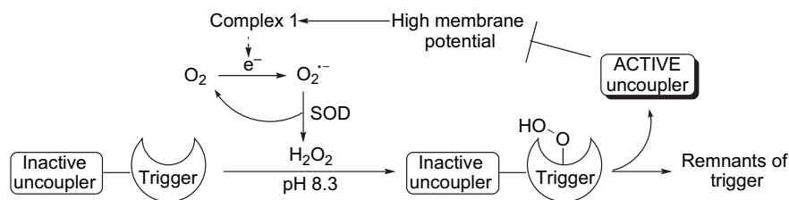
Scheme 1. Proposed mode of action of caged uncouplers.
