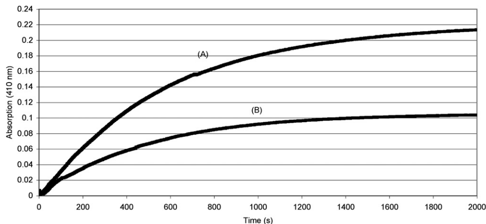
Figure 2. Hydrogen peroxide triggered release of DNP/DNP - from a 200 μM solution of caged uncoupler 15 in 1:1 DMF/aqueous NaHCO 3 monitored by absorbance at 410 nm. Initial concentrations of hydrogen peroxide were 20 μM for line (A) and 10 μM for line (B).
