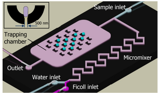
Figure 1: Schematic illustration of the optofluidic chip for biophysical measurement of single bacterium by using null-method in immersion refractometry. Inset shows the trapping structure with a gap of 500 nm.
