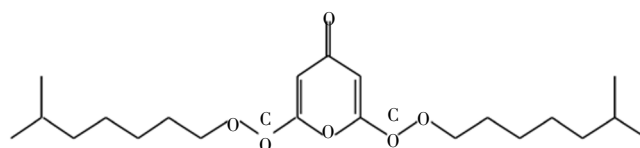
Figure 1. 4-Oxo-4H-pyran-2,6-dicarboxylic acid bis-[6-methyl-heptyl] ester.
