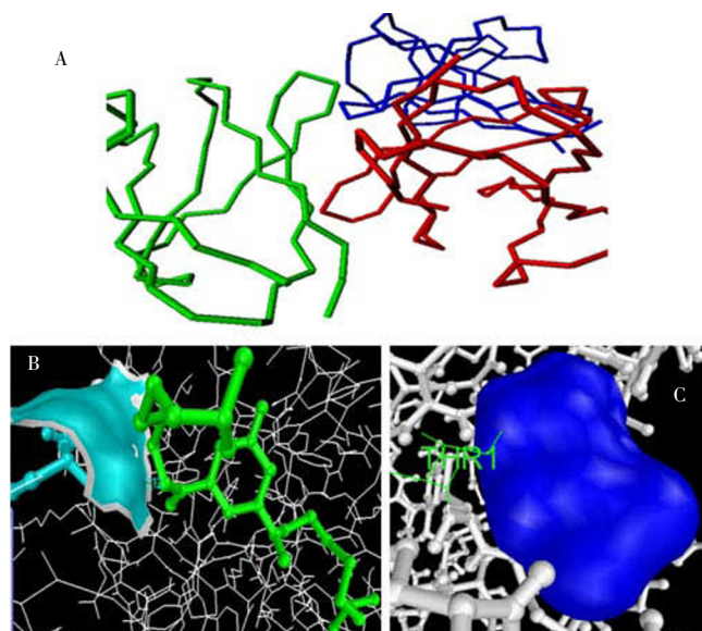
Figure 2. (a) Structure of ampk as seen in proteinscope viewer; (b) orientation of pyran ester in the active pocket of ampk; (c) enfolding of metformin in active pocket.
