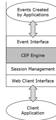
Figure 4 Server architecture.
