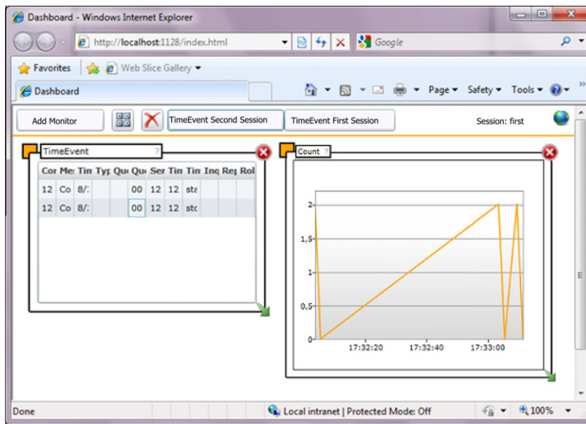
Figure 5 Screenshot of the client application.
