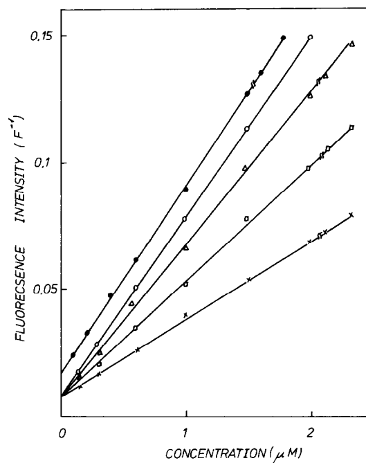
Fig. 3. Two reciprocal coordination plots of fluorescence intensity as a function of rhodamine-B concentration by different molar ratios of L/D ; 0.92 (○), 1.35 (△), 1.64 (□), 2.38 (×). The data were corrected as described in the text. Experimental points for single bilayer liposomes (●).
