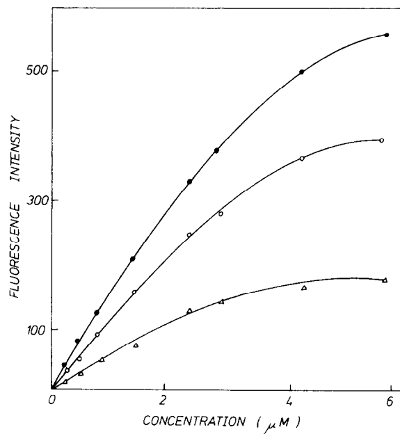
Fig.1. Fluorescence intensity of LBW preparation as a function of the rhodamine-B concentration by different molar ratios of L/D ; 0.54 ( \bullet ), 1.35 ( \circ ), 5.94 ( \Delta ).
