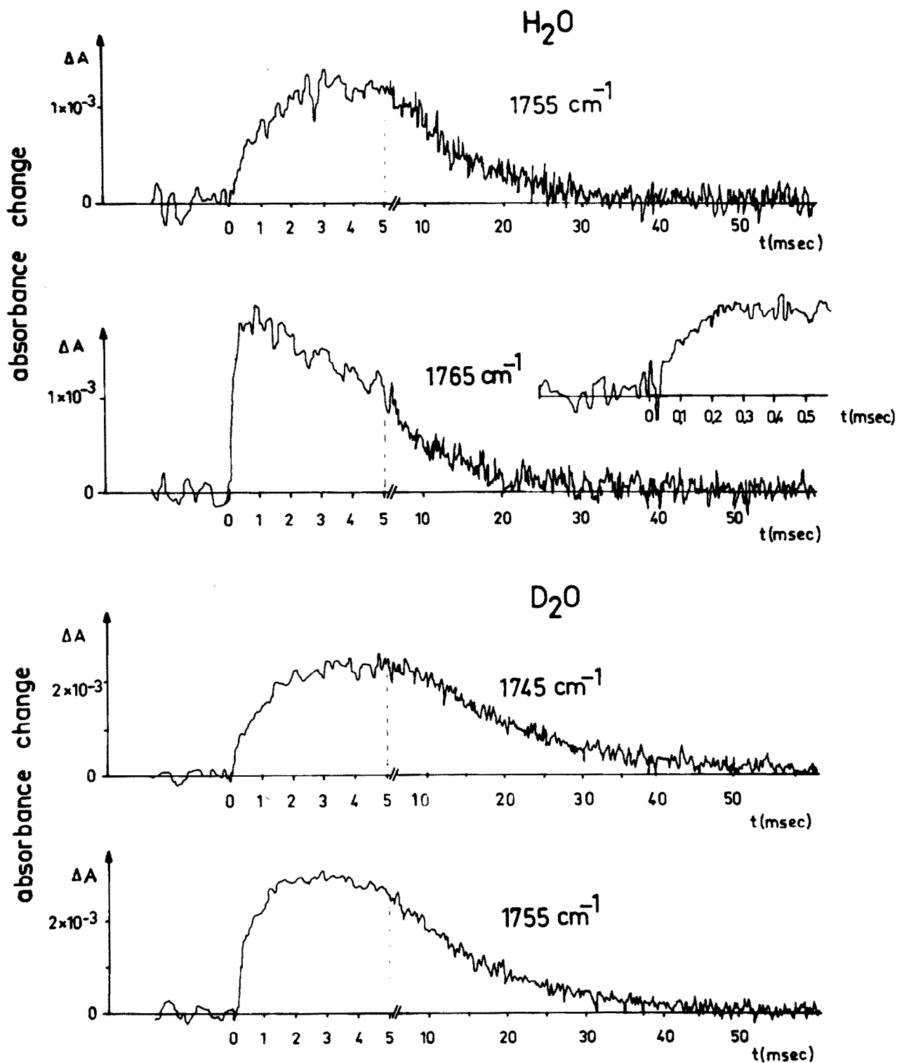
Fig.1. Kinetic signals of a purple membrane film in the hydrated and deuterated state: T = 20^\circ\text{C} , the sample is excited at t = 0 with a Xenon flash at wavelengths > 530 \text{ nm} ; 100 signals were averaged to improve the signal-to-noise ratio. Note change in time base at 5 ms. Insert at 1765 \text{ cm}^{-1} shows time-resolved absorbance rise.
