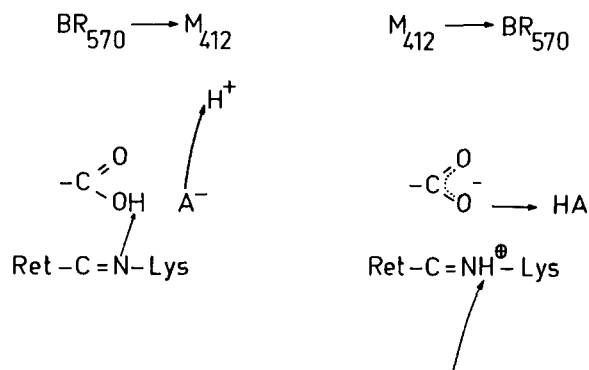
Fig.3. Schematic representation of the molecular steps involving carboxyl group protonation (BR570 \rightarrow M412) and deprotonation (M412 \rightarrow BR570). Abbreviations: Ret, retinal; Lys, retinal-binding lysine
