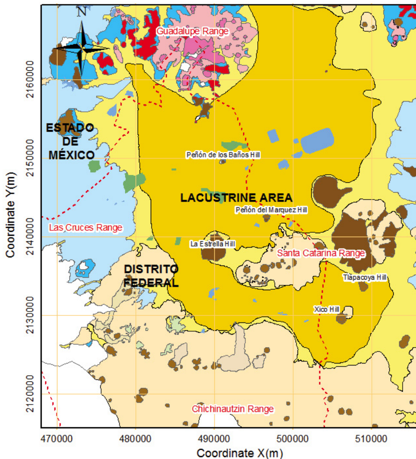
Figure 3. Geology of the study area (Mooser, 1996)
