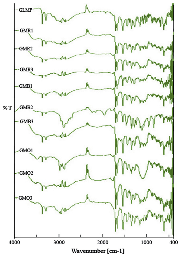
Figure 1 FTIR spectra of pure GLMP and tablet formulations (GMR1 to GMO3).
