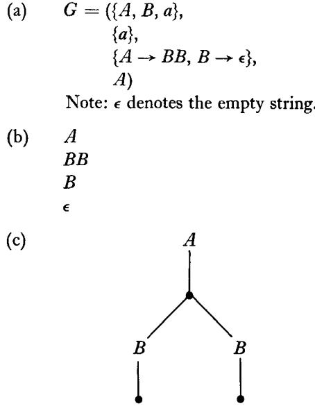
FIG. 1. (a) is a general phrase-structure (more precisely: context-free) grammar; (b) is a derivation of the sentence \epsilon which is, by the way, the unique sentence of this grammar; (c) is the syntactical structure of this sentence. As F(\epsilon, B, B \rightarrow \epsilon) = (BB, B) = F(B, \epsilon, B \rightarrow \epsilon) , the grammar G is not resolvable; the derivation (b) nevertheless defines a single syntactical structure, viz., (c).
