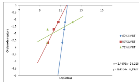
Fig. 7. Weibull parameters Curve – different tension
