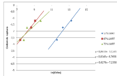
Fig. 4. Weibull parameters Curve – different tension
