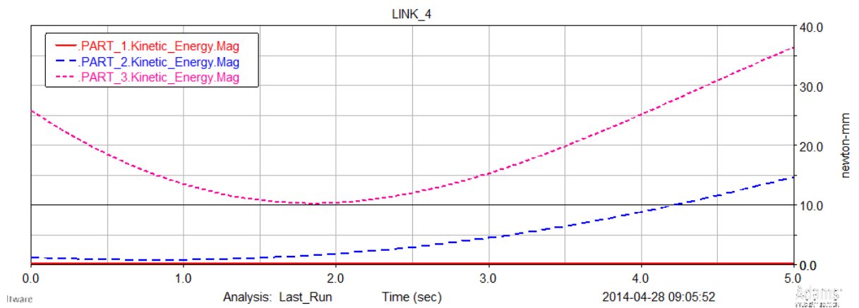
Fig.13 Kinetic energy of links
