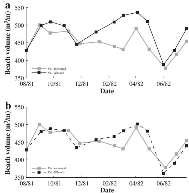
Fig. 8. Comparison of simulated and measured beach volumes from 25/08/81 to 16/08/82. Individual event calibration (a) and annual series calibration (b).
