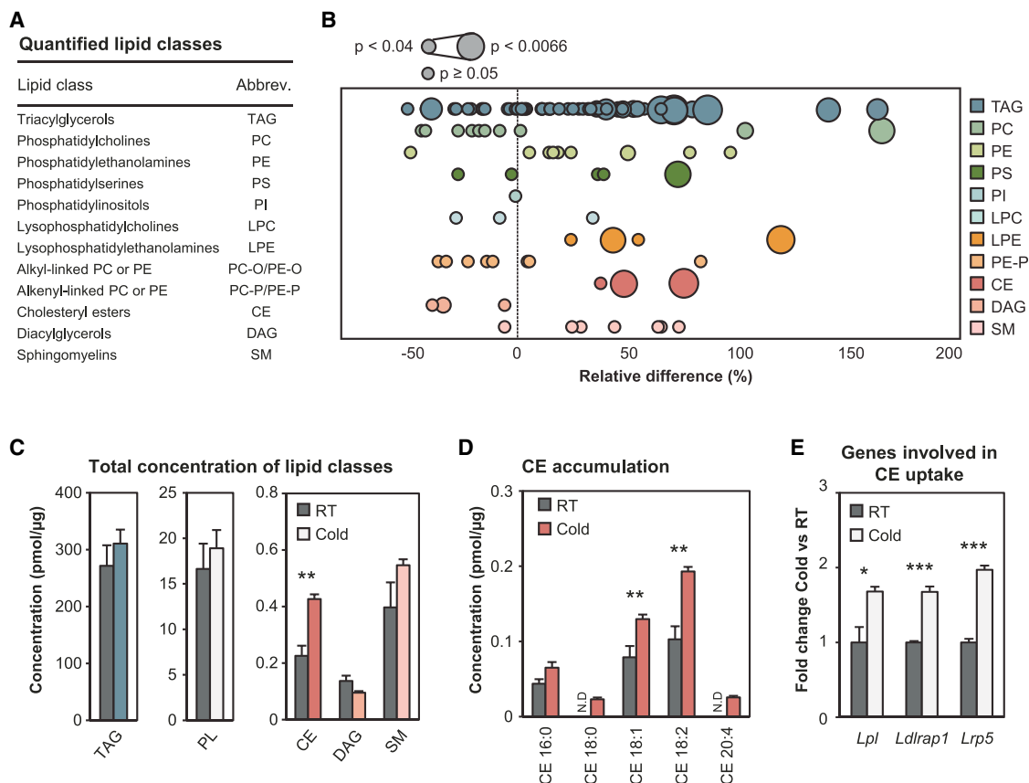
Figure 3. Changes in Overall Lipid Composition of iBAT upon Short-Term Cold Exposure
