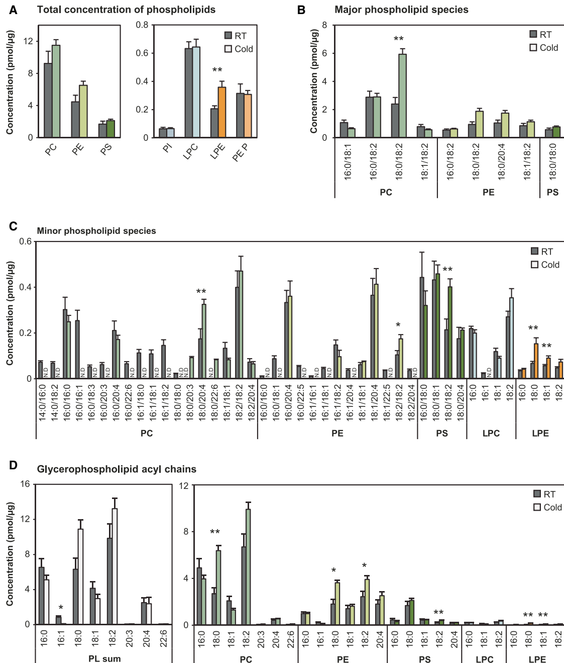
Figure 6. Cold-Mediated Changes in Glycerophospholipid Composition and Fatty Acyl Levels in iBAT
