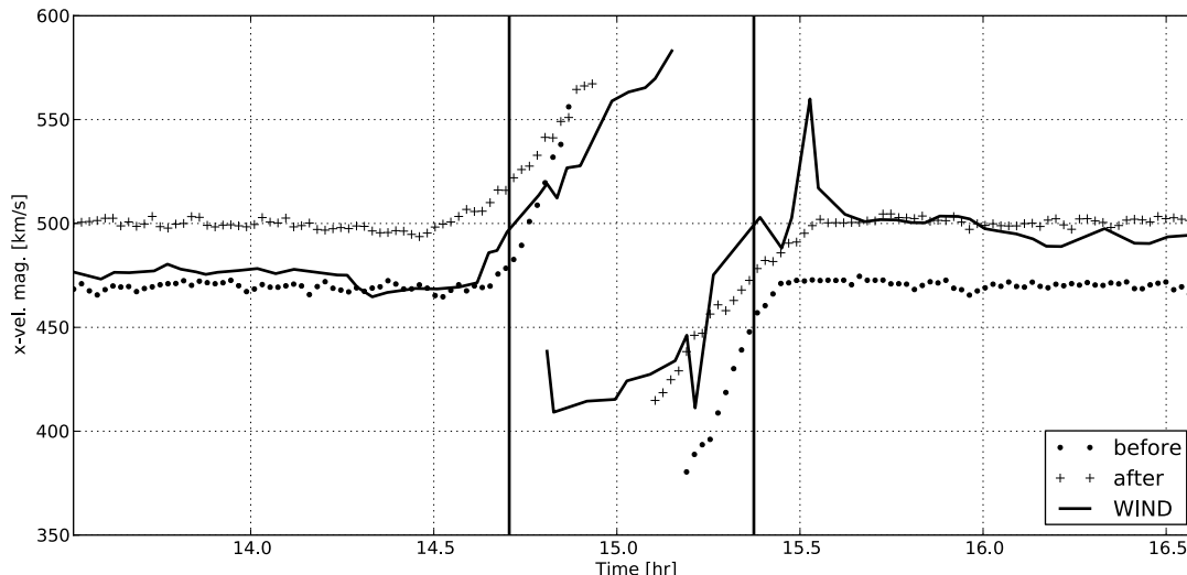
Fig. 7. The hybrid model proton x -velocity magnitude [km/s] for two different upstream solar wind conditions (labeled before and after ), compared to WIND observations. Otherwise similar to Fig. 6. The reason that the WIND velocity is double valued in the center of the wake is that the velocity of the two proton beams refilling the wake from each side is computed separately, as explained in the original publication (Ogilvie et al. , 1996).
