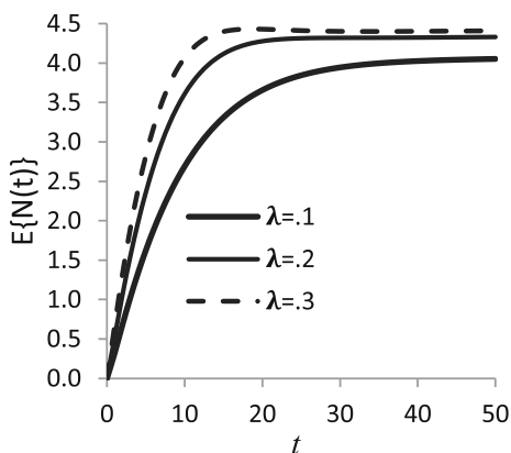
Fig. 6 Variation in E\{N(t)\} for different values of \lambda
