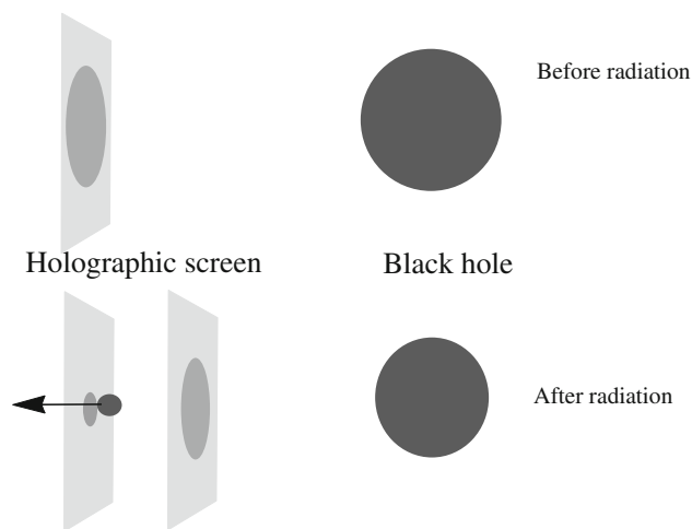
Fig. 1 A schematic drawing of a particle radiated out of a black hole and their holographic screen
