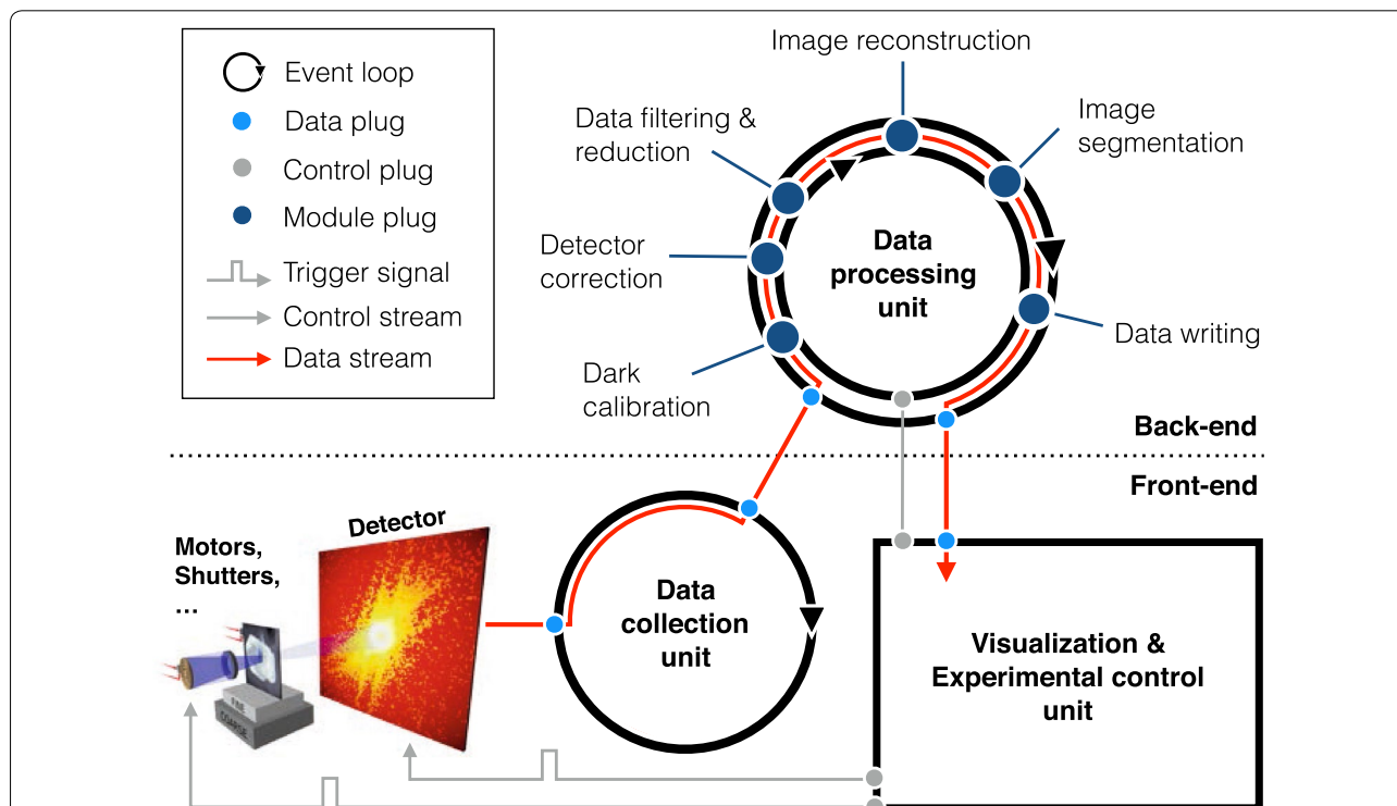
Fig. 1 Streaming pipeline: Overview of the real-time streaming framework of Nanosurveyor. The modular server–client infrastructure is divided into a back-end (running the data processing unit) and a front-end (running the visualization and control unit). The data flow is depicted as a red arrow , while communication channels for controlling experiment and back-end are shown in gray . Once an experiment has started (trigger signal), the data collection unit continuously receives new data packets from a detector and sends raw data frames to the data processing unit. Depending on the specific needs of the experiment, different modules (from dark calibration to data writing) can be plugged into the pipeline. At all times, there is an active connection (asynchronous socket communication) between all components (including the visualization interface) allowing the scientist to monitor progress while data are still being acquired and processed
