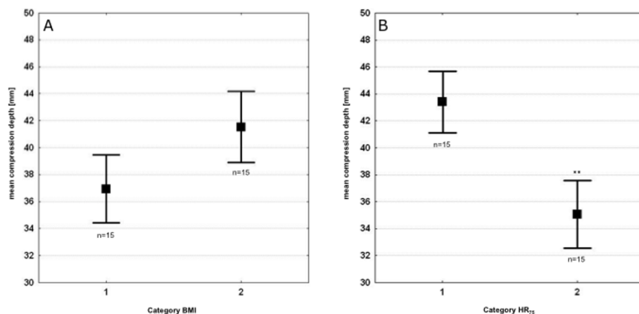
Figure 3 Average compression depth of nine minutes of external chest compression performed by male participants. A: categorised for lower and higher Body Mass Index (BMI); B: categorised for lower and higher heart rate at 75-watt rowing (HR 75 ). Category BMI: 1 = participants with lower BMI; 2 = participants with higher BMI; Category HR 75 : 1 = participants with lower HR 75 ; 2 = participants with higher HR 75 ; **: p < 0.05. Data are presented as mean ± standard error of mean. For the definition of lower and higher HR 75 and BMI, respectively, please refer to the main text.
