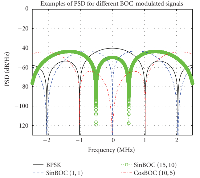
FIGURE 2: Examples of baseband PSD for BOC-modulated signals.
