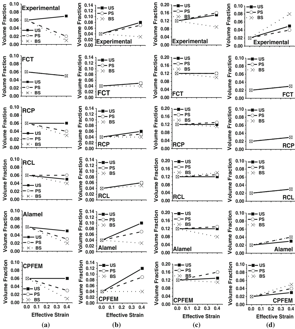
Fig. 5—Volume fractions estimated from experimental (Fig. 2) and simulated (Fig. 4) ODFs for ideal fcc texture components [67] of (a) cube \{001\}\langle 100\rangle , (b) Cu \{112\}\langle 111\rangle , (c) S \{123\}\langle 634\rangle , and (d) Brass \{110\}\langle 112\rangle .
