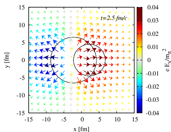
Fig. 1. Electric field generated in the transverse plane of Cu+Au collisions at \sqrt{s_{NN}} = 9 GeV, b = 4.5 fm and t = 2.5 fm/c. The direction of the arrows indicates the field direction projected onto the reaction plane and the length is proportional to the electromagnetic strength shown in color.
