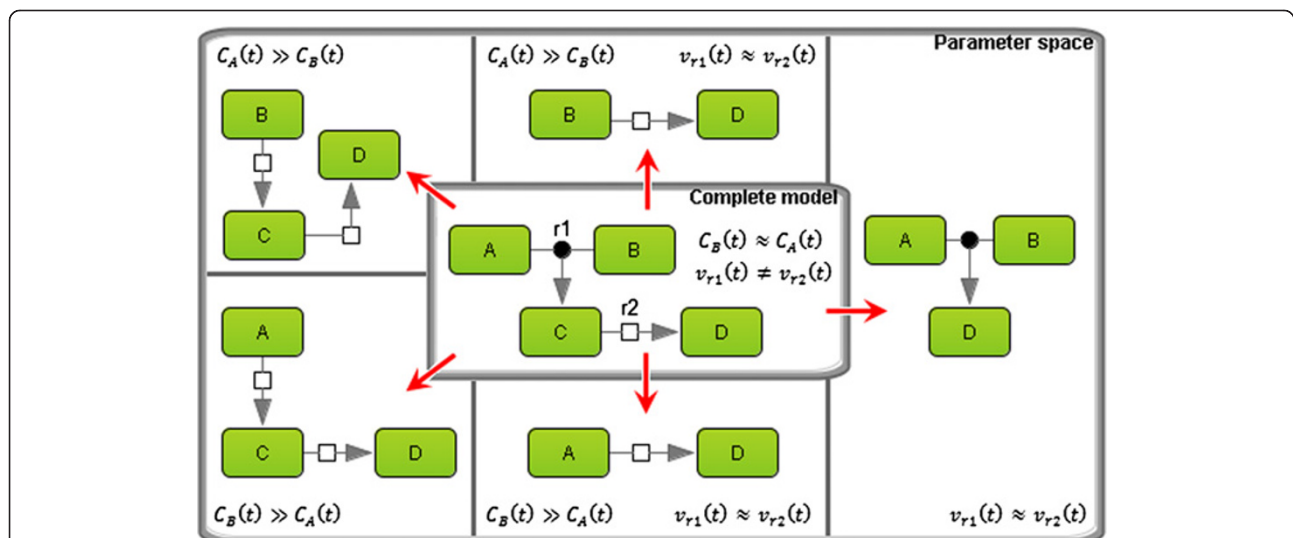
Figure 1 Schematic representation of the model reduction technique. A model consisting of four species ( A , B , C , and D ) and two reactions ( r_1 and r_2 ) was reduced taking into account the relations between time-dependent concentrations C_A(t) and C_B(t) , as well as reaction rates v_{r1}(t) and v_{r2}(t) . In the case when C_A(t) \gg C_B(t) , the concentration of A can be considered constant for some period of time. The same simplification could be applied to B . If v_{r1}(t) \approx v_{r2}(t) , then C could be removed, resulting in direct formation of D triggered by the binding of A and B only.
