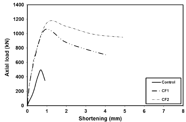
Fig. 8 Experimental results of load-shortening curves of strengthened columns using steel-casing
