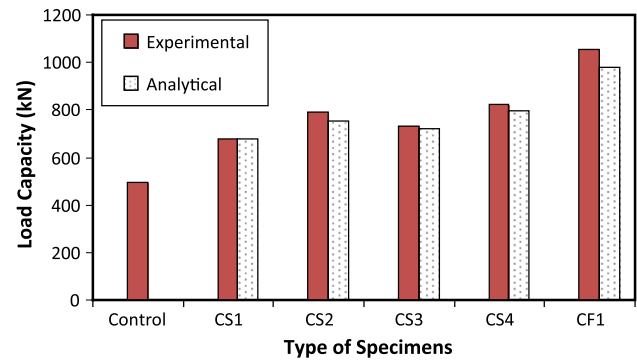
Fig. 22 Comparison between experimental observed results with analytical results
