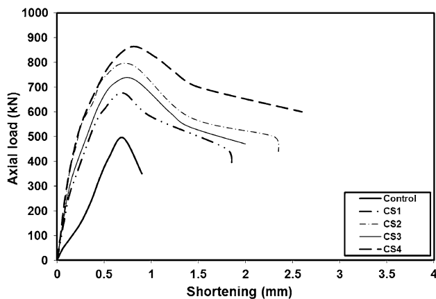
Fig. 7 Experimental results of load-shortening curves of strengthened columns using steel angles with strips
