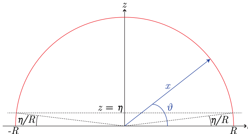
Figure 2. Mapping the z = \eta cut-off to polar coordinates. The red semicircle is the entangling surface while the location of \mathcal{O}_\Sigma is at z = 0 . A uniform cut-off z = \eta close to the location of \mathcal{O}_\Sigma is introduced. It is denoted with a dashed horizontal line. This limits integration over \vartheta between \eta/R and \pi - \eta/R .
