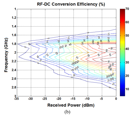
Fig. 17. (a) Measured output DC power of the rectenna as a function of the received RF power and frequency. (b) Measured conversion efficiency of the rectenna
