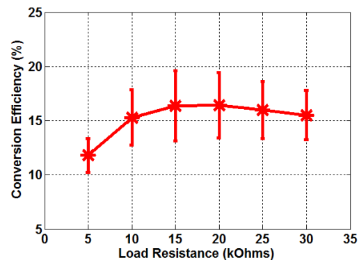
Fig. 21. Measured overall conversion efficiency versus different load with error bar
